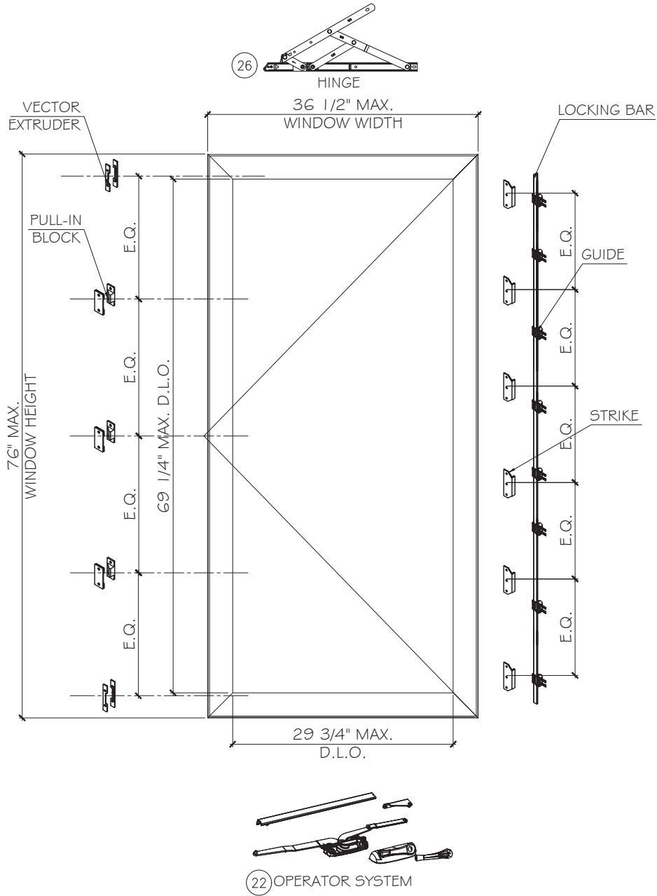
HARDWARE LAYOUT
